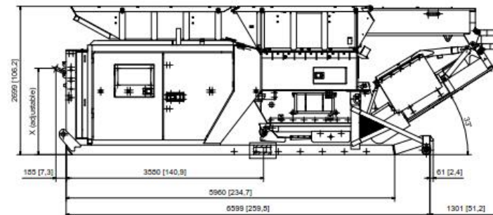
TRANSPORT POSITION
